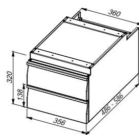
Double drawer block: plain/frame for GN 1/1 container Code: Y-STP2/Y-SGN2
