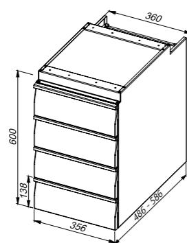
Quadruple drawer block: plain/frame for GN 1/1 container Code: Y-STP4/Y-SGN4
