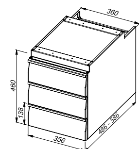
Triple drawer block: plain/frame for GN 1/1 container Code: Y-STP3/Y-SGN3
