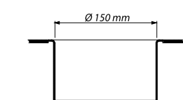
Stainless steel waste hole (ø150, ø200 or ø250 mm) Code: Y-SNA-150
