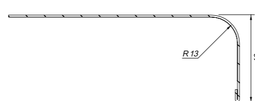
Rounded front edge Code: Z-UP
