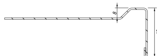
Deepened table top Code: DG
