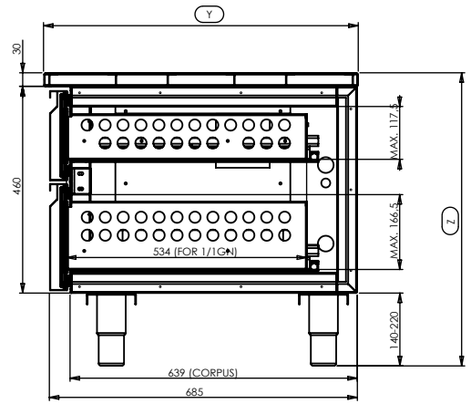
CUT B-B
