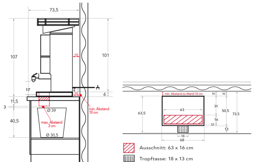
Sample picture: Countertop Installation Kit sectional view 8000 SB
