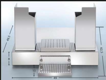
Countertop Installation Kit Art. no.: 70878 Inclusive peel bucket 40 l
