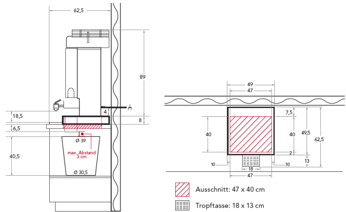
Sample picture: Countertop Installation Kit sectional view 7000 SB
