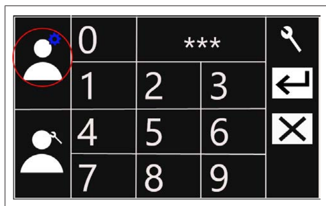
Fig. 20: Logg inn
