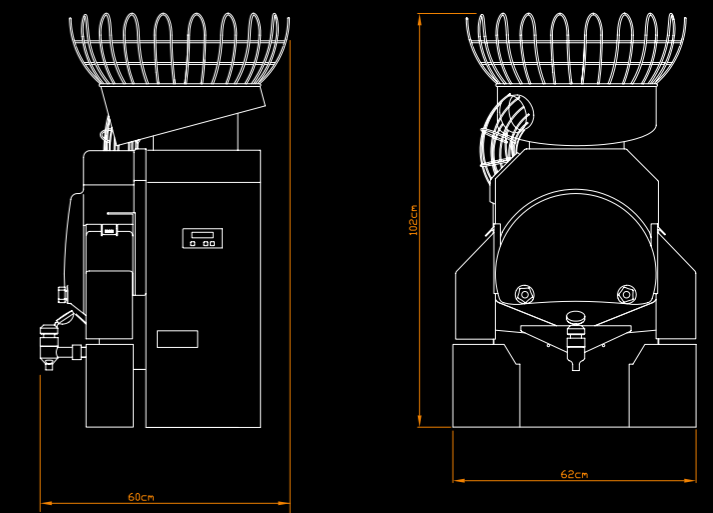
CITROCASA 8000 SB ADVANCE – Technical specifications
