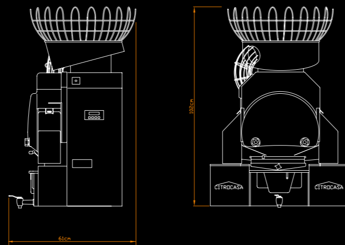
CITROCASA 8000 XB ADVANCE – Technical specifications
